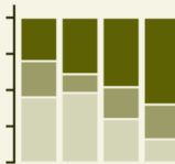
Stacked Bars
