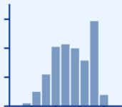
Histogram
