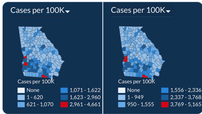
Figure: Total number of COVID19 cases in Georgia, US: July 2 vs. July 17
