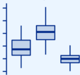
Boxplots
